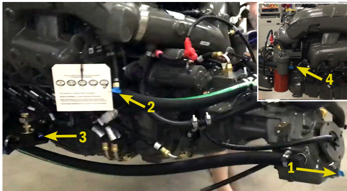
The engine drain plugs are located: 1. The V-drive. 2. The bank 1 manifold. 3. Under the heat exchanger. 4. The bank 2 manifold.
